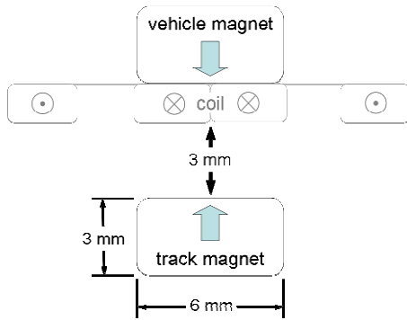
Figure 5. The track and vehicle magnet configuration.
