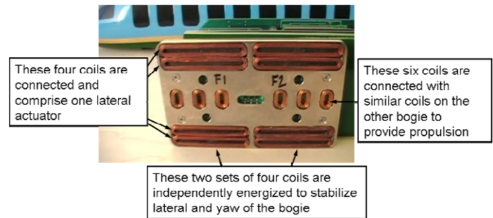
Figure 7. The bottom of the bogie houses the actuator coils and sensors.
