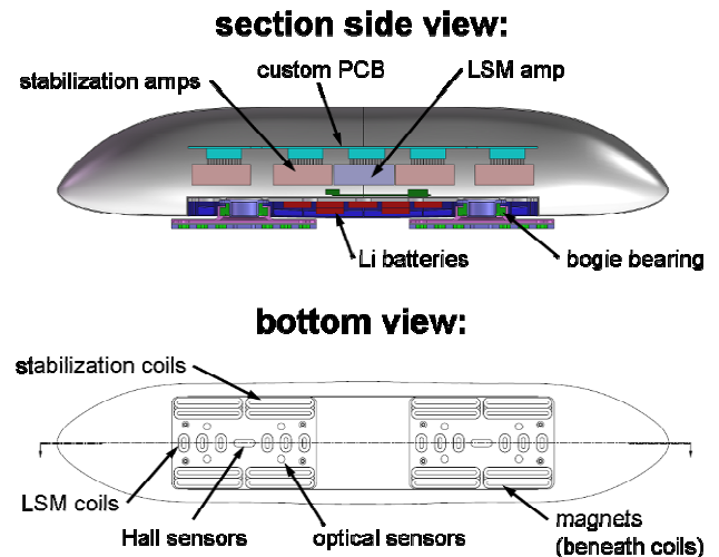
Figure 4. Two views showing several key components.
