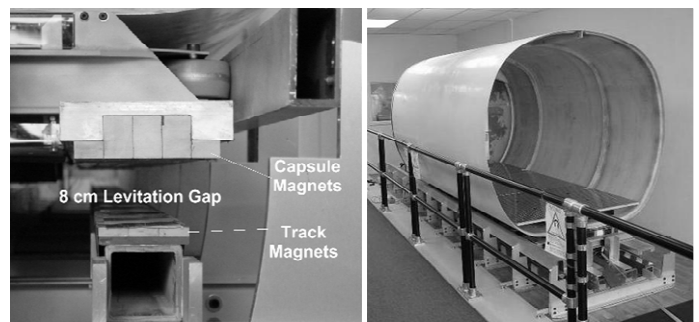
Figure 1. Large-scale permanent magnet demonstration vehicle.
