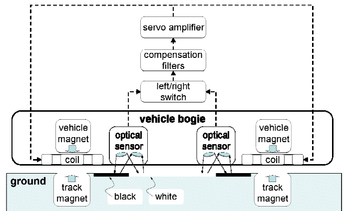
Figure 6. The elements of the lateral stabilization loop.
